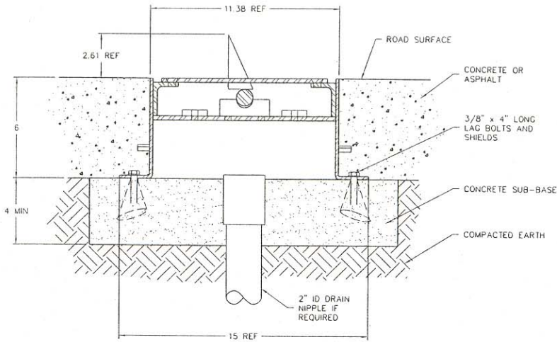
SECTION DETAIL
