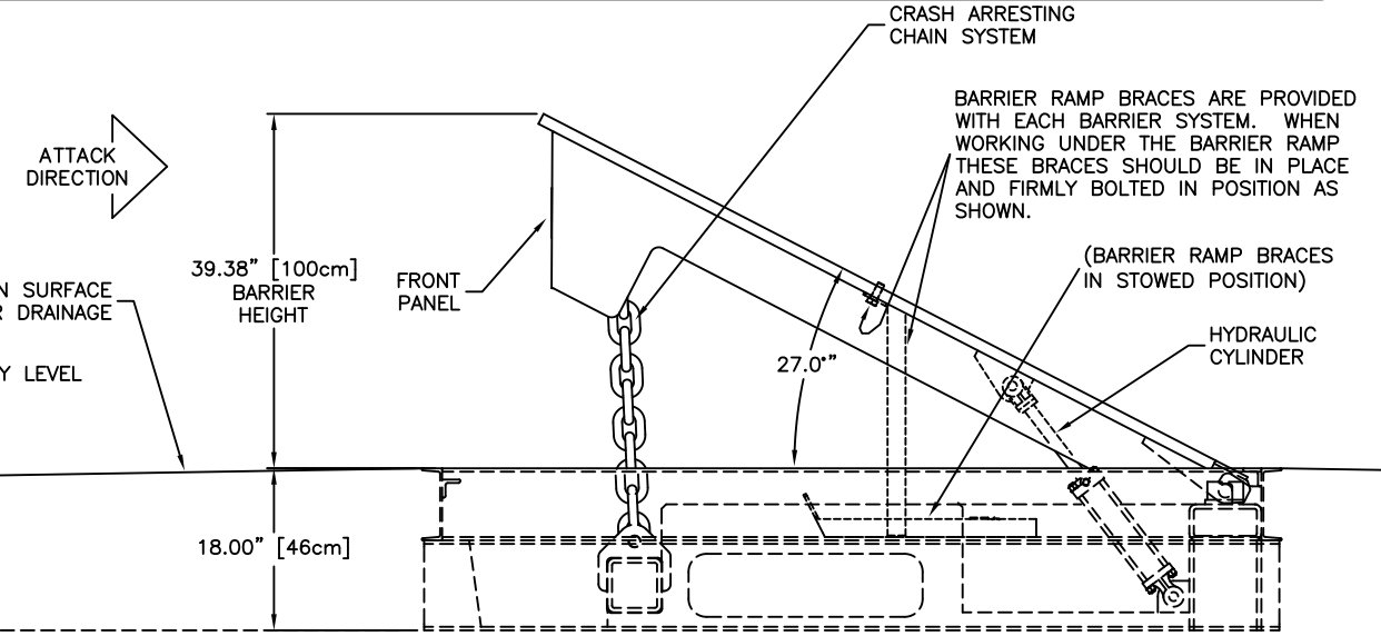
SIDE ELEVATION - UP POSITION
