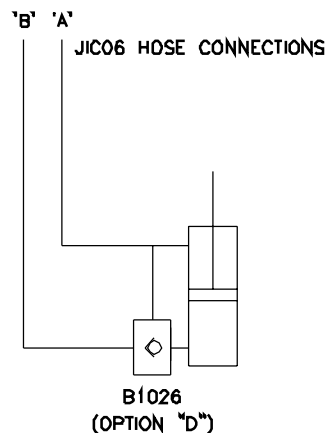
FLOW SCHEMATIC
